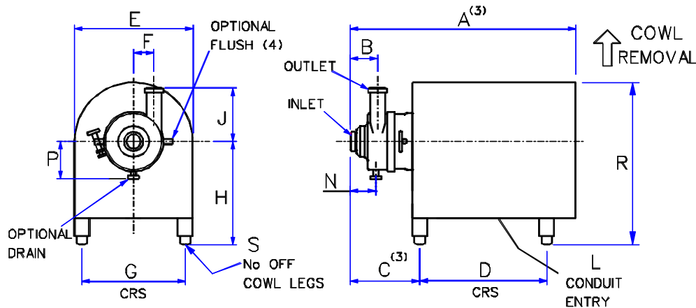
COWLED PUMP
