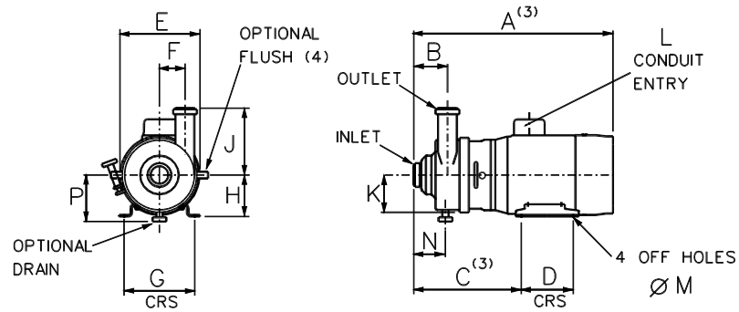
STANDARD PUMP
