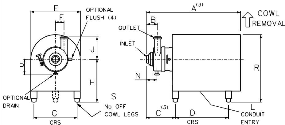
COWLED PUMP
